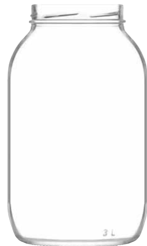
mer300 jar, v: 3000 cc, 101 1/2 oz h: 244 mm, 9 3/5 in, Ø: 100 TO
